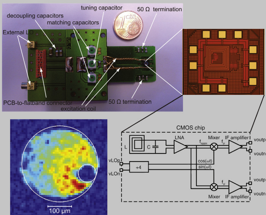
A fully integrated IQ receiver for NMR microscopy. Jens Anders, Paul SanGiorgio, Giovanni Boero. Pages 1-7
